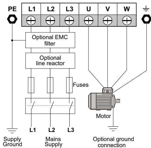
Typical Power Connections
