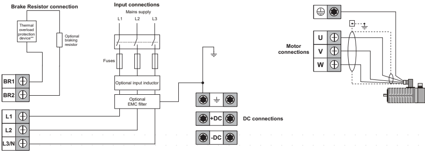
Typical Power Connections
