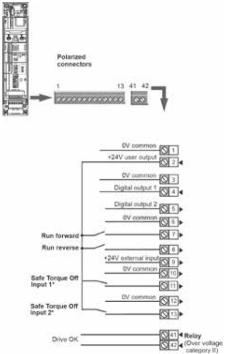
M702: Default Control Connections
